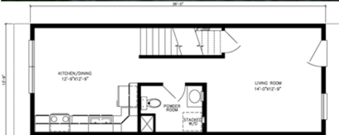
FIRST FLOOR
